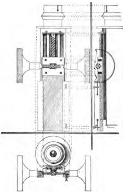
FIG. 42.—Coarse adjustment.
